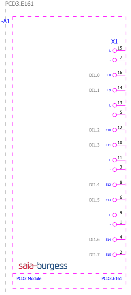
Saia-Burgess\PCD3 Module\PCD3.E161.ema Overview Variant B 2012-10-26 / 2.1.4
