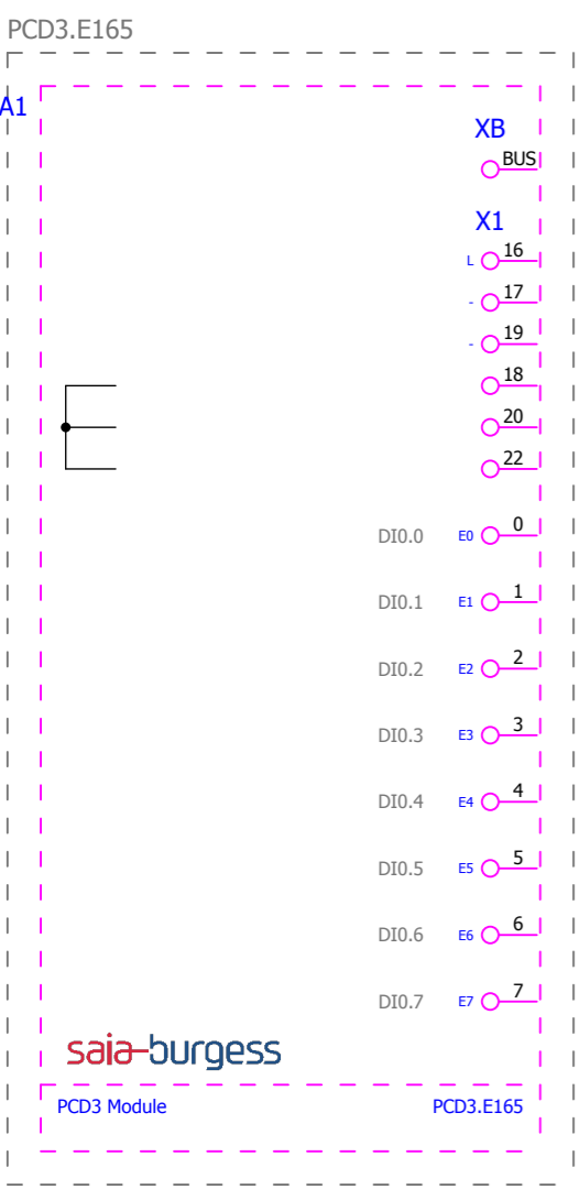
Saia-Burgess\PCD3 Module\PCD3.E165.ema Overview Variant A 2012-10-26 / 2.1.4
