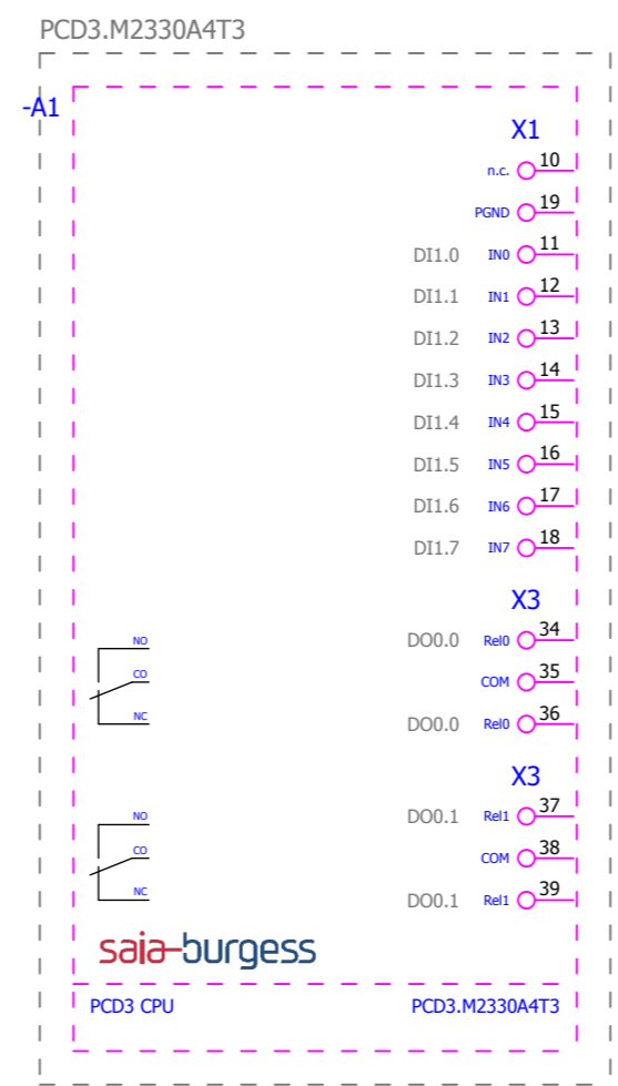
Saia-Burgess\PCD3 CPU\PCD3.M2330A4T3.ema Overview Variant B 2012-10-26 / 2.1.4
