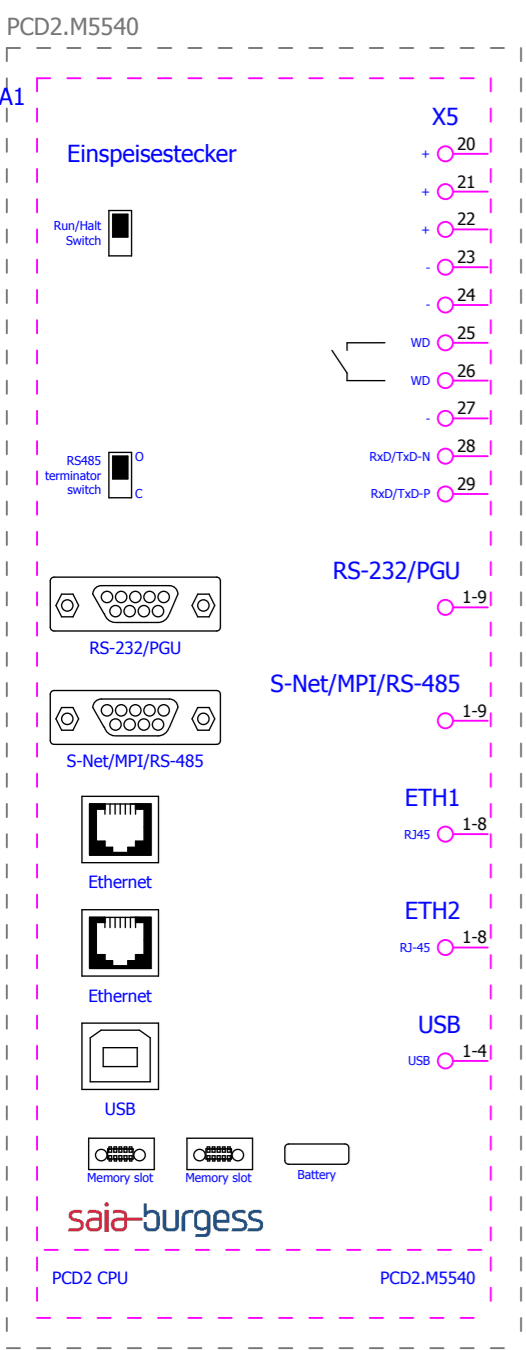
Saia-Burgess\PCD2 CPU\PCD2.M5540.ema Overview Variant A 2012-10-26 / 2.1.4
