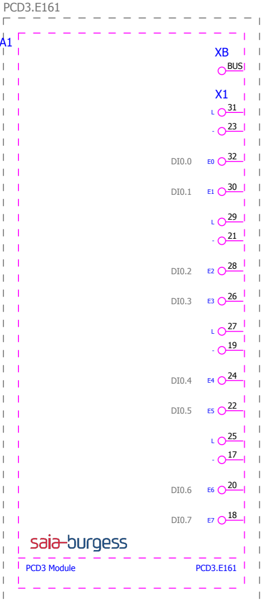
Saia-Burgess\PCD3 Module\PCD3.E161.ema Overview Variant A 2012-10-26 / 2.1.4
