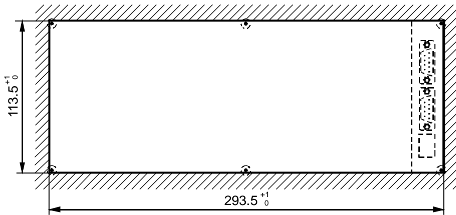
Panel cutout
