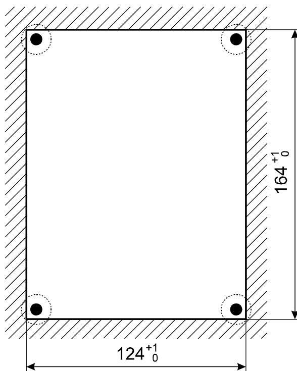
Panel cutout
