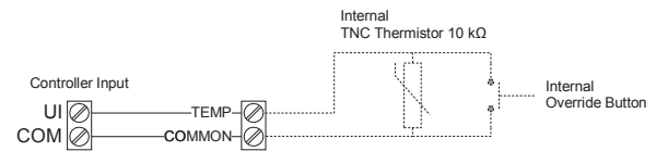
Figure 3: 10 kΩ NTC Thermistor input
