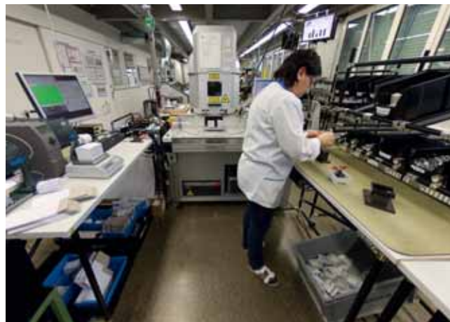
The same production configured as lean: A single person can create a complete product in a few minutes – from the assembly of the printed circuit board to packaging for dispatch.
