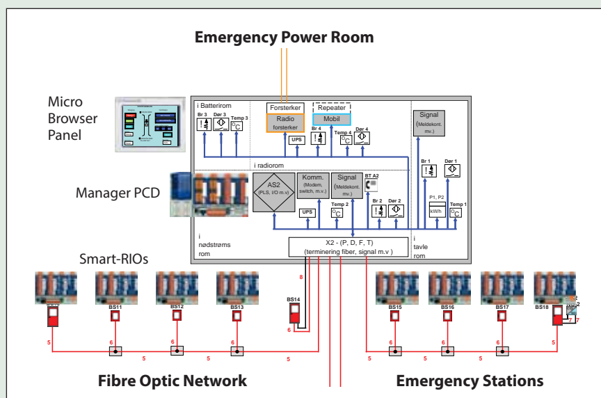
▲ More than 80 Saia®PCD3.T665 Smart RIOs are used in the emergency stations of a road tunnel in Norway for monitoring telephones, fire extinguishers etc.
