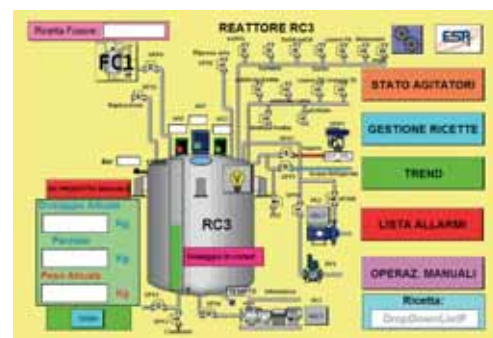
▲ Screenshot of the web-HMI for the chemical reactor, created with Saia® WebEditor 5.14
