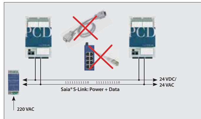
▲ Schematic diagram of "Saia-S-Link": System design with Saia® PCD1. Communication happens without a dedicated cable connection.
