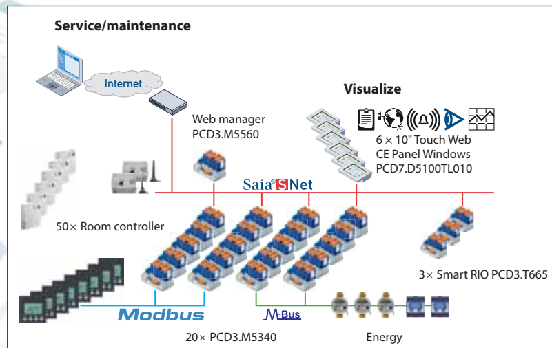
▲ Network topology building technology at MarcCain Saia®PCD3.M5560 Power-CPU with AutomationServer as the central Manager-Station for operation and service.
