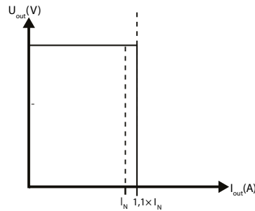
Output Characteristic (U/I Characteristic)
